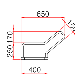
SIDE ELEVATION SCALE : NONE
